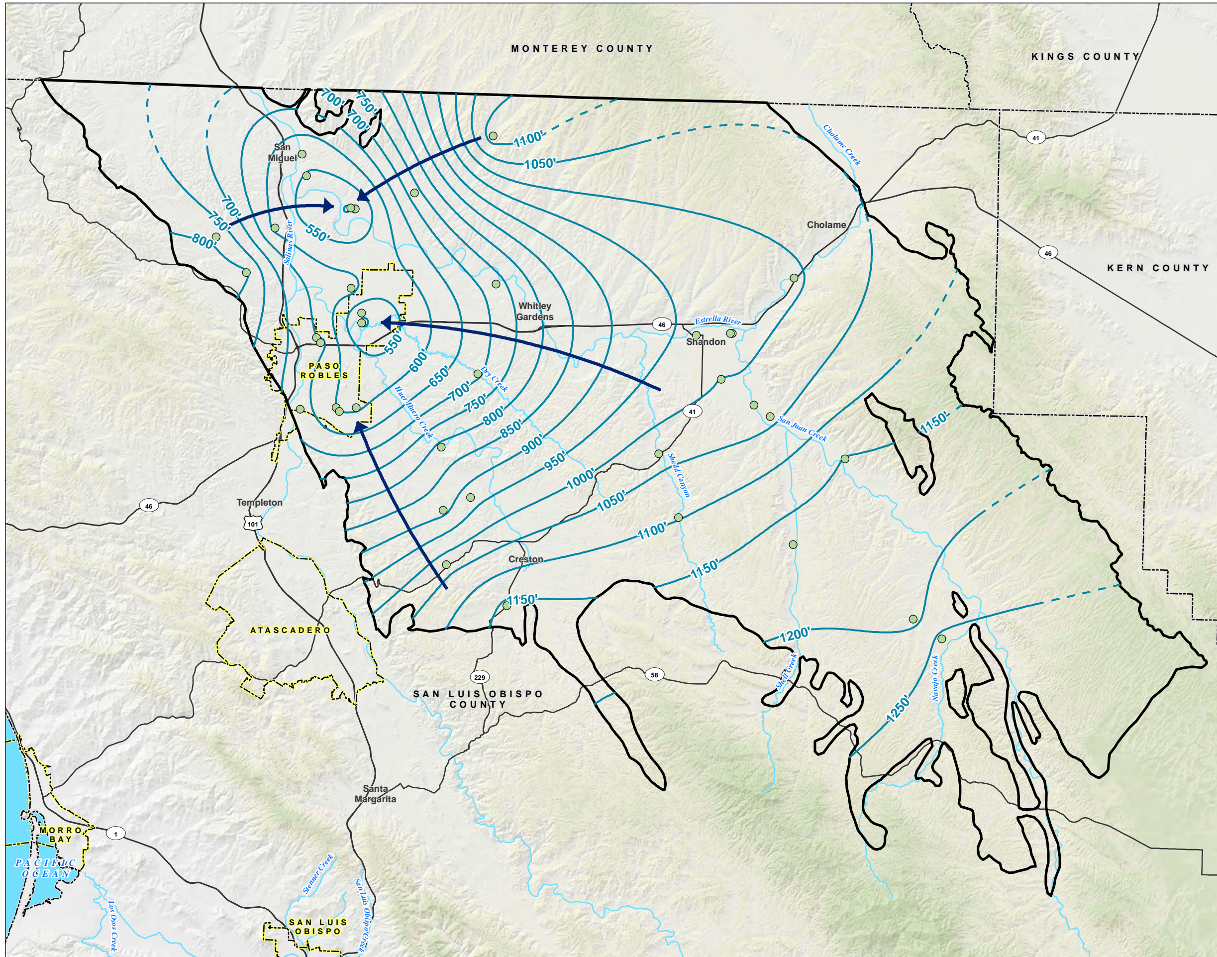
FIGURE 8 Paso Robles Formation Aquifer Spring 2019 Groundwater Elevation Contours Paso Robles Subbasin First Annual Report
