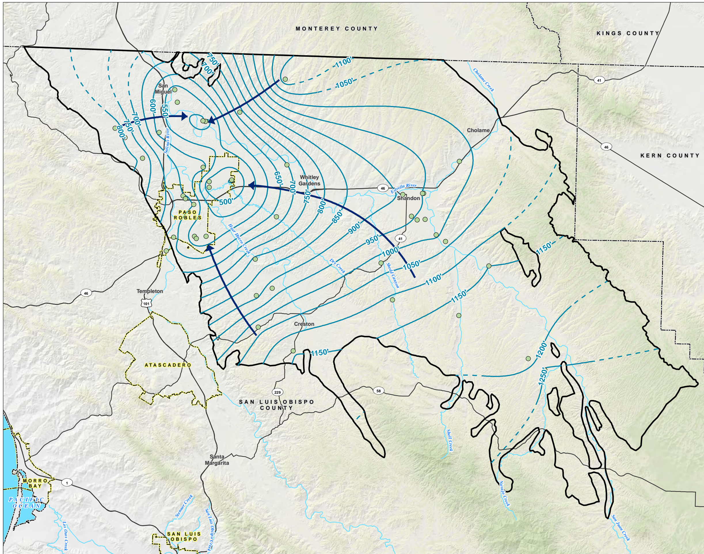
FIGURE 5 Paso Robles Formation Aquifer Fall 2017 Groundwater Elevation Contours
