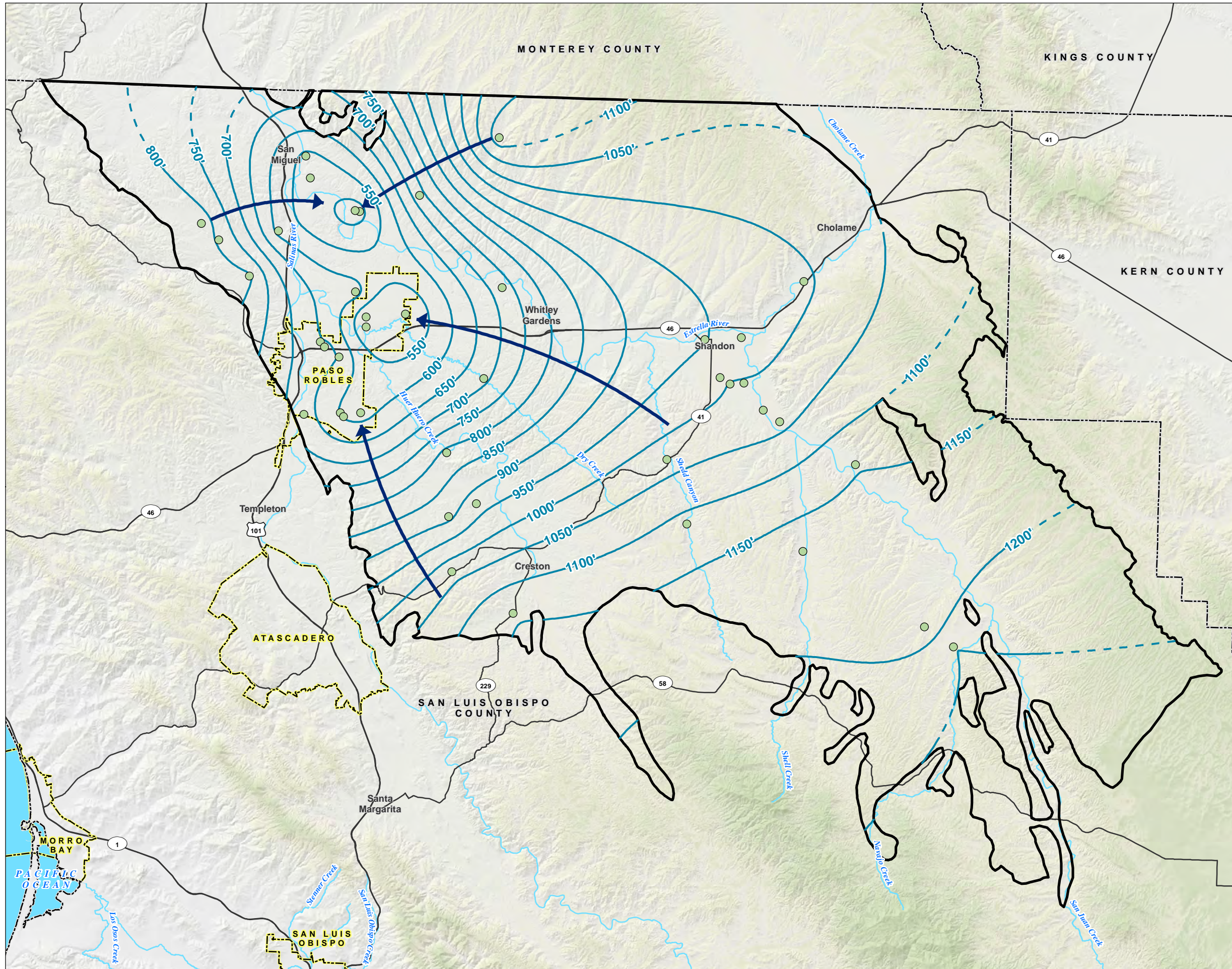
FIGURE 6 Paso Robles Formation Aquifer Spring 2018 Groundwater Elevation Contours Paso Robles Subbasin First Annual Report
